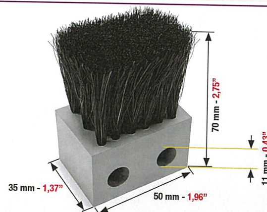
SPAZZOLA LUBRIFICA CATENE BRUSH FOR CHAIN LUBRICATION CEPILLO LUBRICA CADENAS
