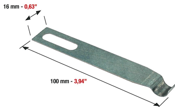
SEPARATORE CARTA- EXPERTCUT-MASTERCUT SPRING SEPARATOR PAPER- EXPERTCUT-MASTERCUT MUELLE SEPARADORA PAPEL- EXPERTCUT-MASTERCUT
