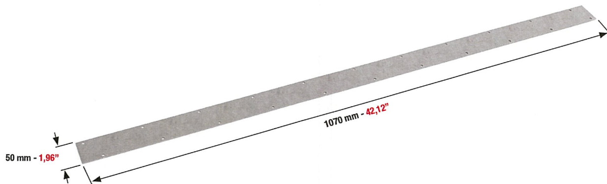
MOLLE PER TAPPETO "NON-STOP" "NON-STOP" SPRINGS FOR APRON MUELLE "NON-STOP" PARA EXPULSION DE LA HOJA
